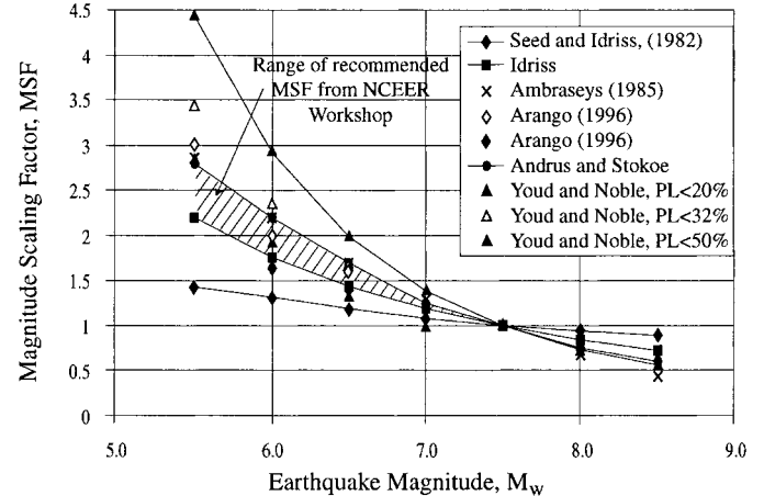
FIG. 12. Magnitude Scaling Factors Derived by Various Investigators (Reproduced from Youd and Noble 1997a)
