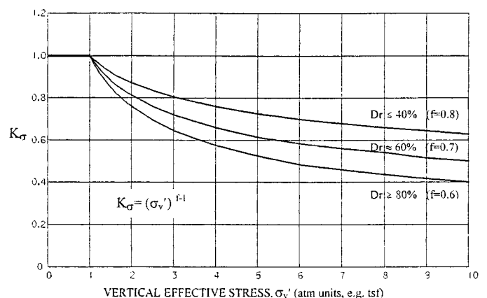
FIG. 15. Recommended Curves for Estimating K_\sigma for Engineering Practice
