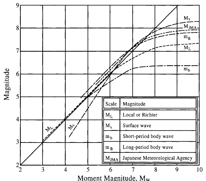
FIG. 16. Relationship between Moment M_w and Other Magnitude Scales (Reproduced from Heaton et al. Unpublished Report, 1982)
