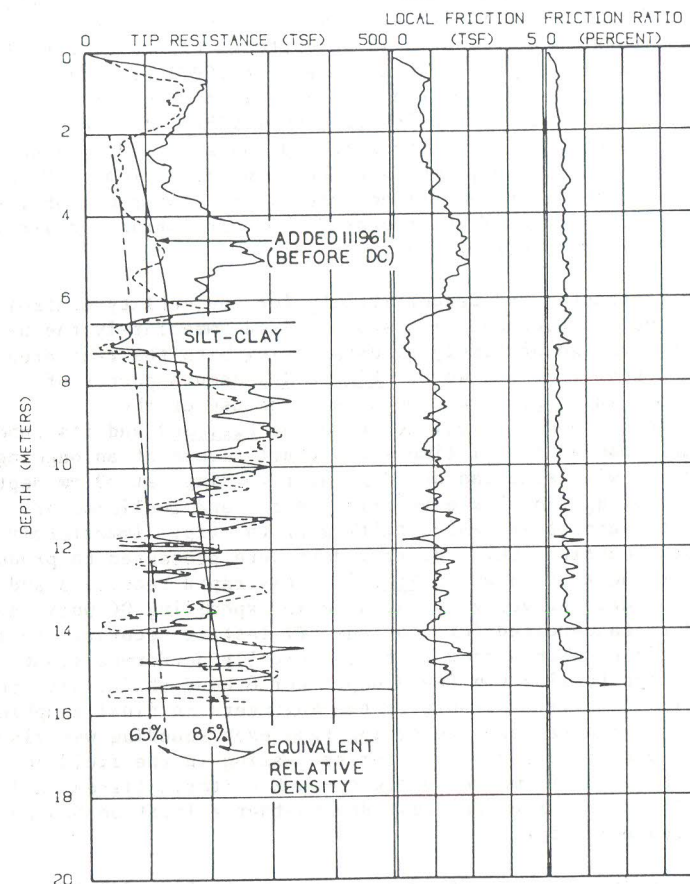
FIGURE 4 - EXAMPLE OF CPT LOG PRODUCED DIRECTLY IN THE FIELD, ANNOTATED
