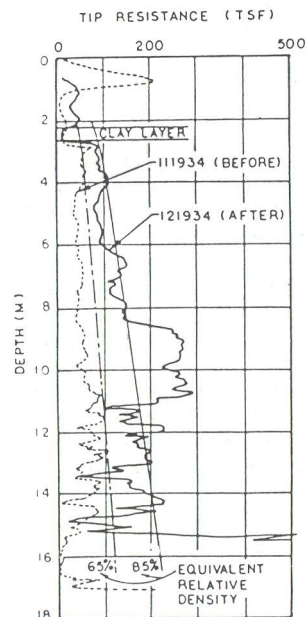
FIGURE 5b - GRAPHICAL LOG FOR SELECTED OUTPUT IN FIG. 5a, INCLUDES BEFORE-AFTER COMPARISONS
