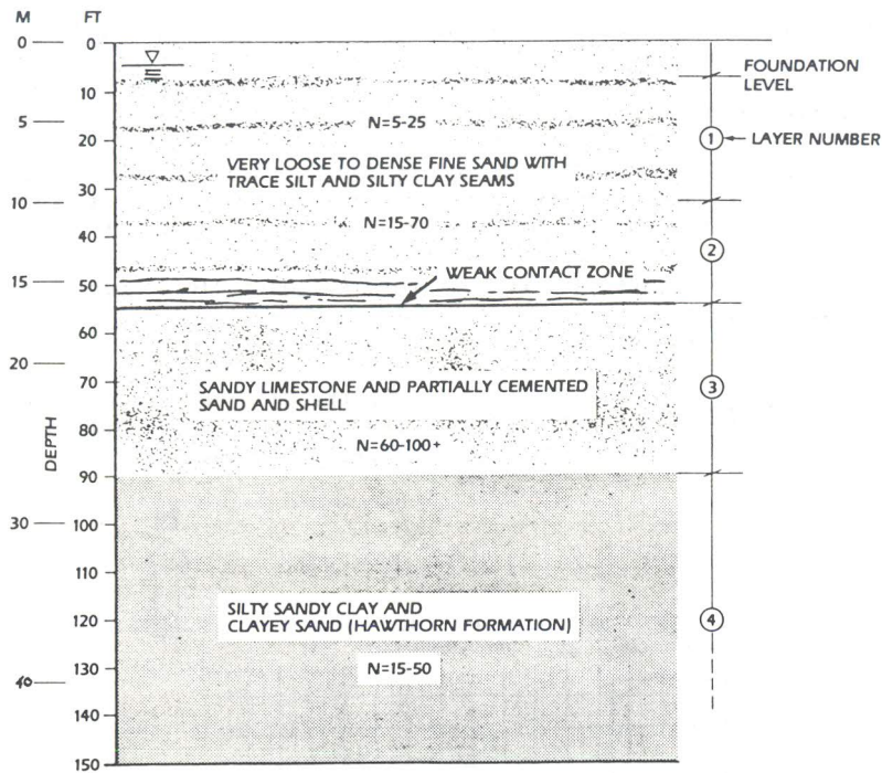
FIGURE 1 - GENERALIZED SUBSURFACE PROFILE
