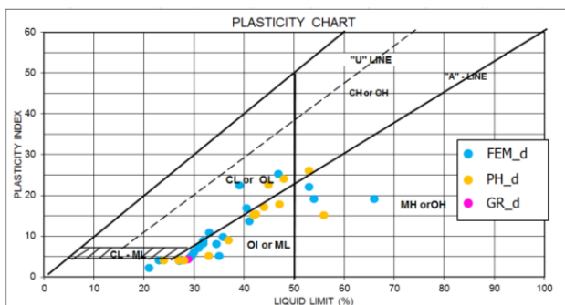
Fig. 6 – Plasticity Index summary graph
