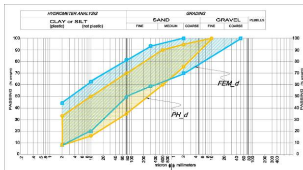
Fig. 5 – Residual soils grading from femic and phillite
