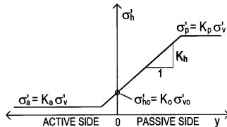
Fig. 1. Typical pressure-displacement relation of the springs
