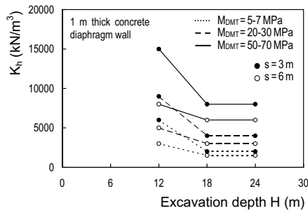
Fig. 5. "Best fit" K_h vs excavation depth H for different values of constrained soil modulus M_{DMT} and prop spacing s
