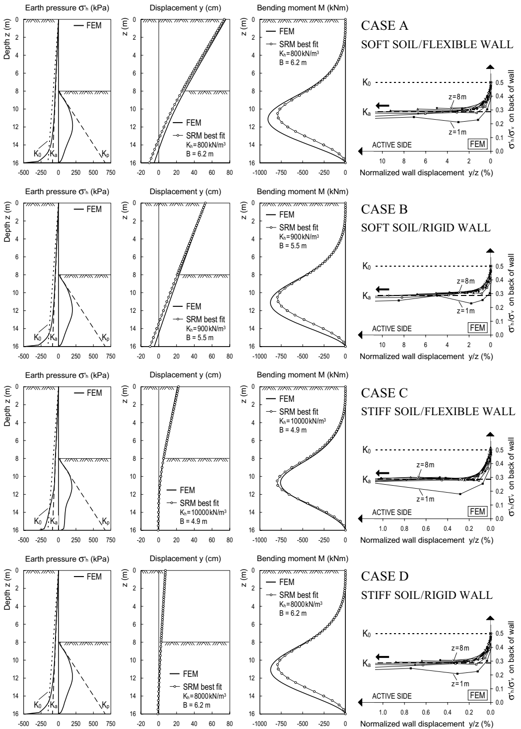
Fig. 8. Results of FEM and SRM analyses for cantilever wall. Earth pressure distribution, horizontal wall displacements and bending moments at 8 m excavation depth. Normalized pressure–displacement curves on back of wall at 1 m depth intervals.
