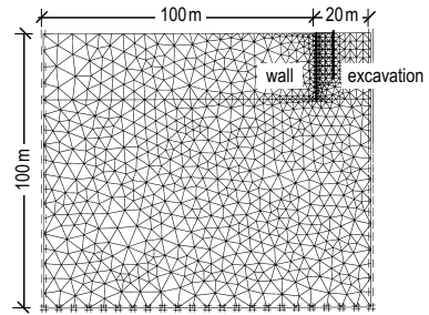
Fig. 3. Finite element mesh for multi-propped wall study
