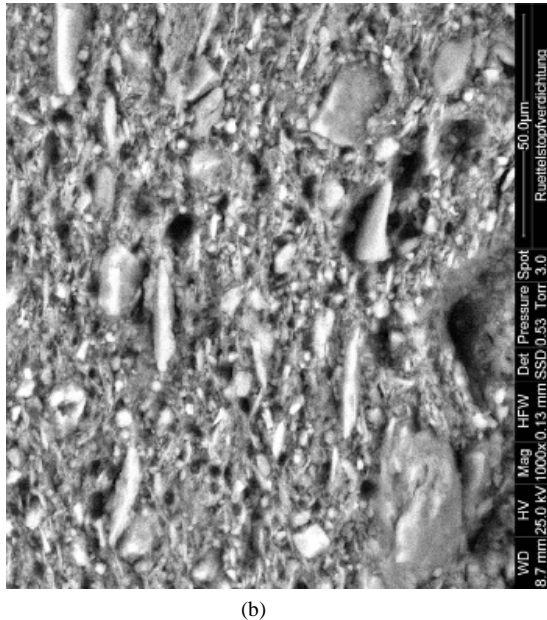
Figure 3.22. Environmental Scanning Electron Microscopy of the zone around the sand compaction pile: (a) showing the indentation of sand particles into the clay, and successively less disturbed zones in the clay; (b) 120x120 \mu\text{m} ESEM picture at from the centre of the box in a) (Weber et al. 2009).
