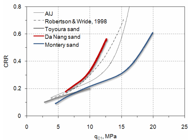
Figure 5.6 Comparison of the CRR- q_{c1} correlations derived for three clean sands (after Ishihara and Harada, 2008).
