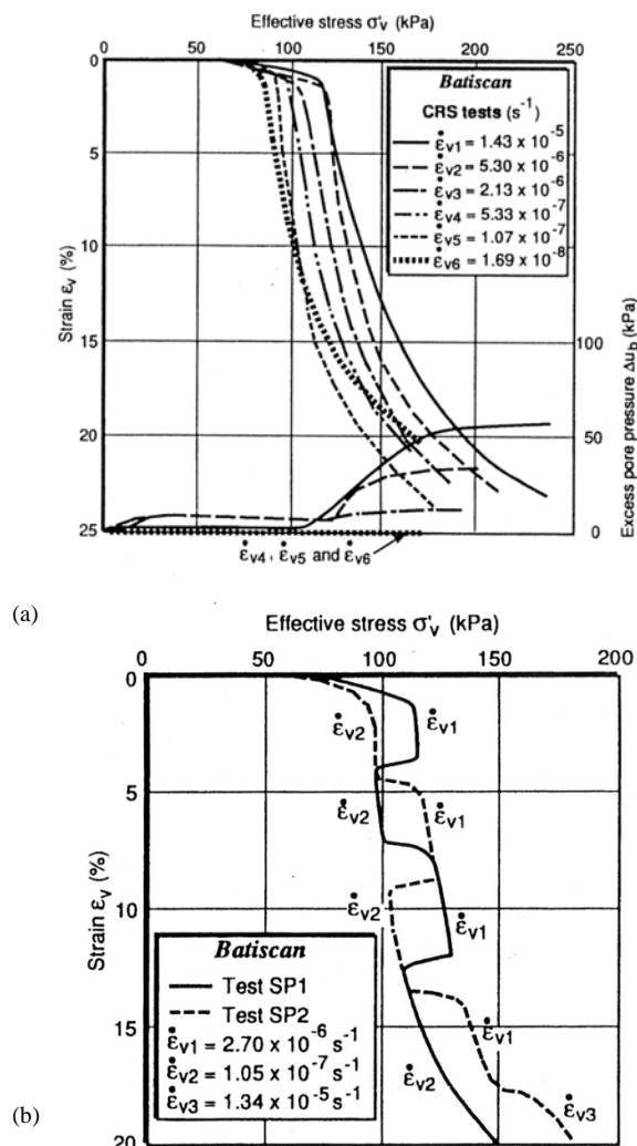
Figure 2.29. Typical oedometer test data for a soft clay (a) Constant Rate of Strain tests (b) Step-changed Rate of Strain test (Batiscan clay, Leroueil et al. 1985).
