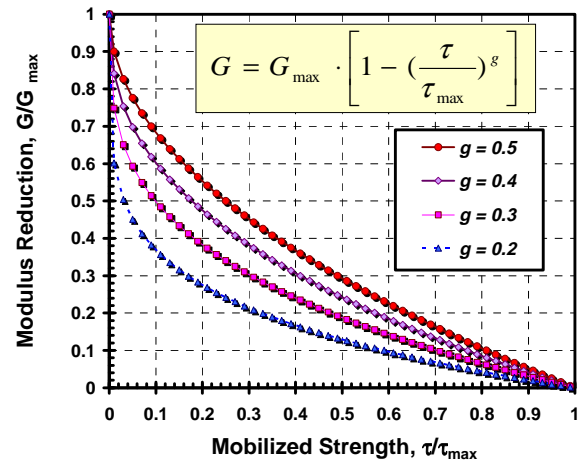
Figure 4.31. Algorithm for modulus reduction curves in terms of mobilized shear stress for “hourglass” sands and “vanilla” clays.
