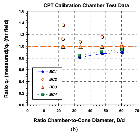
Figure 3.3. Calibration chamber size effect for cone penetration resistance a) for Hoksund sand with R_d = ratio of chamber to cone diameter (after Parkin & Lunne 1982) and b) for Ticino and Toyoura sand (Iwasaki et al. 1988).
