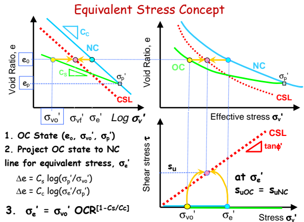
Figure 1.33. Equivalent stress concept in CSSM spaces.
