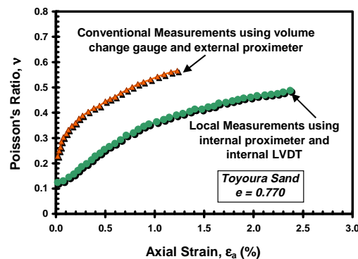
Figure 1.21. Conventional external vs. local internal measurements of Poisson's ratio (data from Jamiolkowski et al. 1994).
