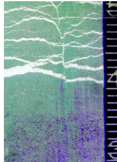
Figure 3.23. Devon silt frozen from the top, with fluorescent tracer showing saturated zone at the base, frozen fringe and ice lens formation (Arenson et al. 2008).
