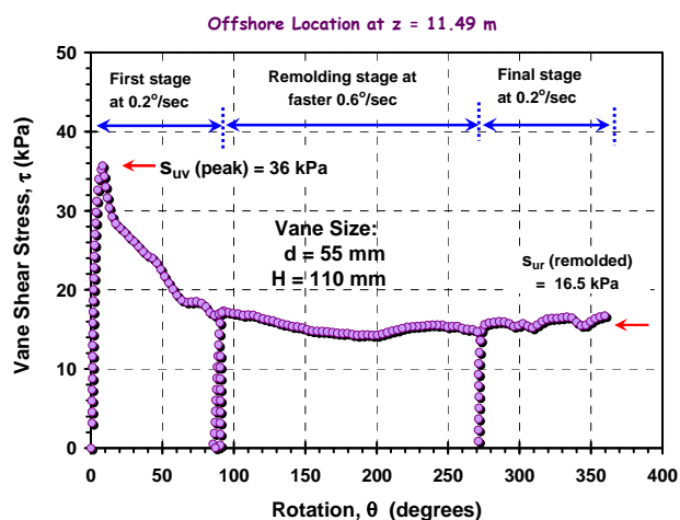
Figure 4.35. Electrovan tests in clay from offshore site in Eurasia (Peuchen & Mayne 2007).
