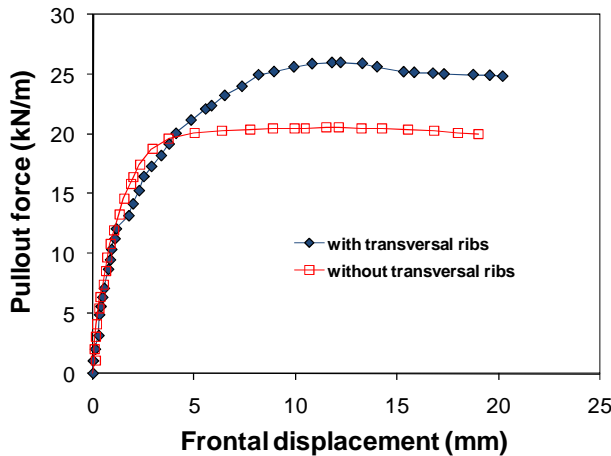
Figure 6.4. Results of pullout tests conducted using geogrids with and without transverse ribs (Teixeira et al. 2007).
