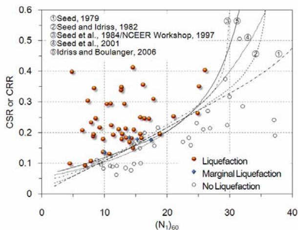
Figure 5.1 CRR- (N_1)_{60} correlations published in the past 3 decades for clean sands (after Idriss and Boulanger, 2006).
