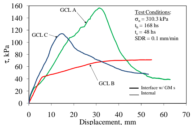
Figure 6.9. Shear stress-displacement curves for different GCLs: GCLs A (needle-punched), B (stitch-bonded), and C (thermally-locked) (Zornberg et al. 2005).
