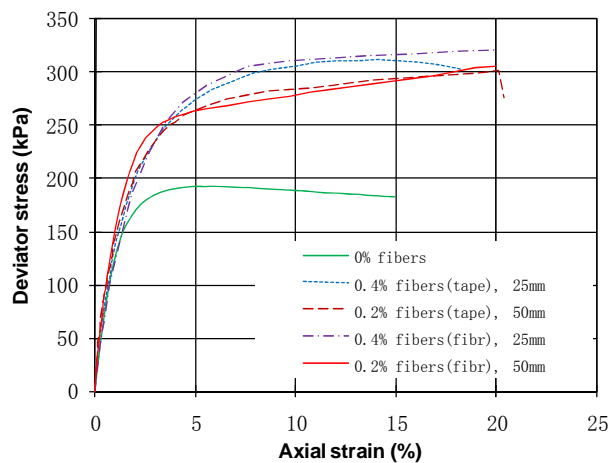
Figure 6.19. Stress-strain behavior for specimen reinforced with 50mm-long fibers placed at a fiber content of 0.2% and 25 mm fibers placed at a fiber content of 0.4%, \sigma_3 = 70 kPa (Zornberg and Li 2003).
