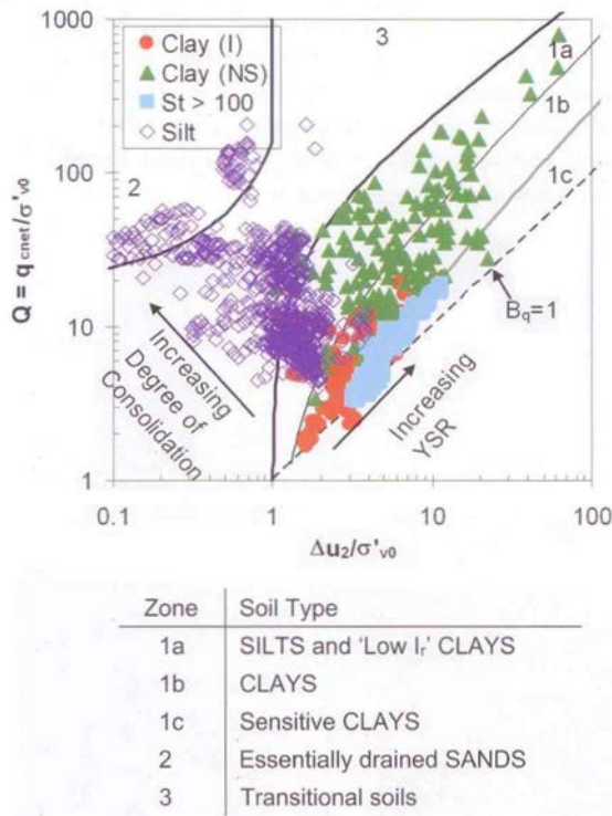
Figure 4.11. New CPT soil behavioral type chart using Q and normalized porewater pressure U^* = \Delta u_2/\sigma'_{v0} (Schneider et al. 2008).
