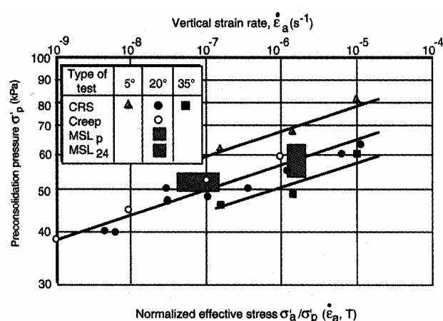
Figure 2.30. Dependency of preconsolidation pressure on rate of loading for Berthierville clay (Boudali et al. 1994).
