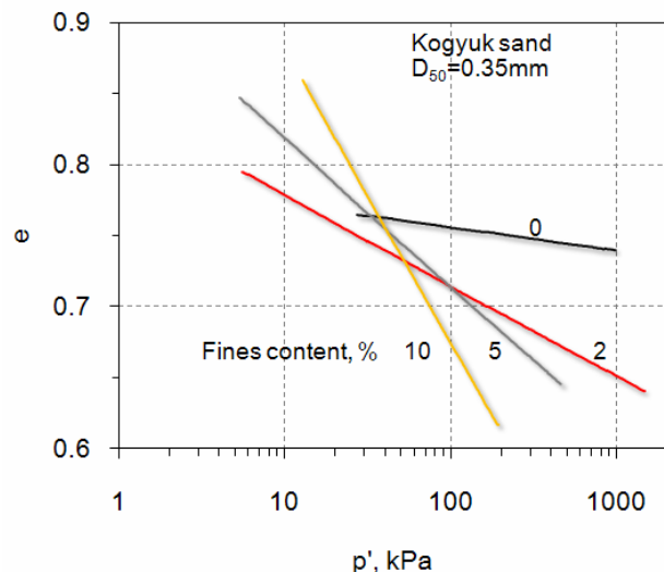
Figure 5.7 Critical state lines for Kogyuk 350 sand with different silt contents (from Been &amp; Jefferies, 1985).
