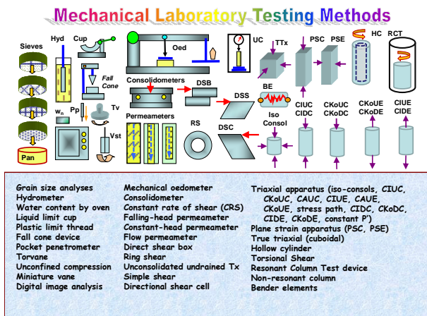
Figure 1.4. Laboratory testing devices for soil parameter determination.
