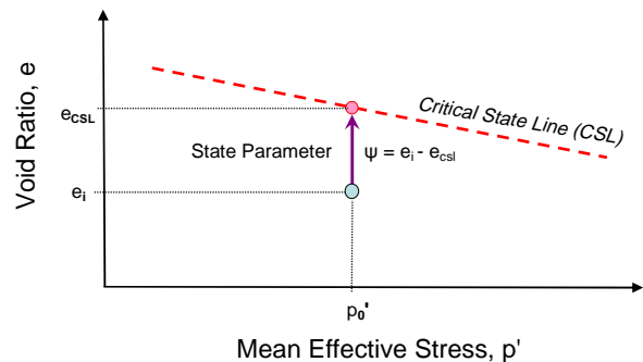
Figure 1.40. State parameter defined for sands in CSSM framework (after Jefferies &amp; Been 2006).
