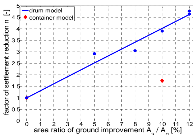
Figure 3.34. Settlement reduction factor determined for embankment crest with drum model representing 3D boundary conditions and the container model, plane strain (Weber 2007).
