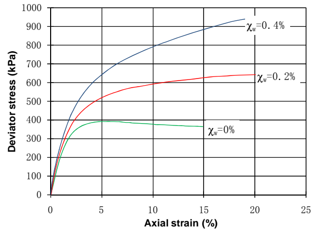
Figure 6.16. Stress-strain behavior of specimens prepared using fiber contents of 0.0, 0.2 and 0.4% with 25 mm-long fibers, \sigma_3=140 kPa (Zornberg and Li 2003).
