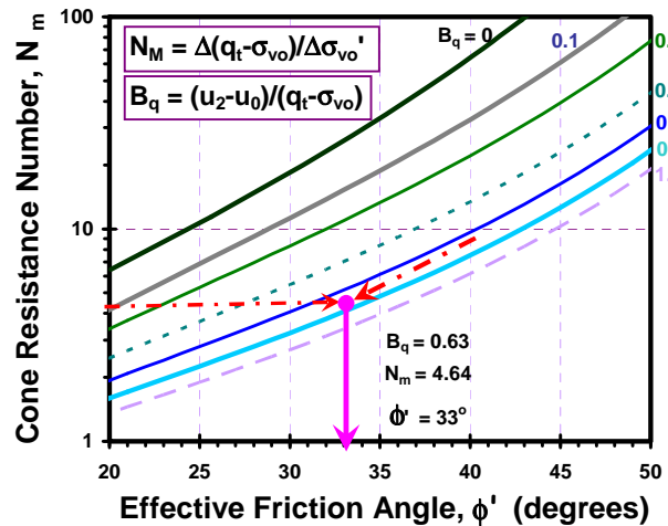
Figure 4.23. NTN method for obtaining \phi' from CPTu parameters.
