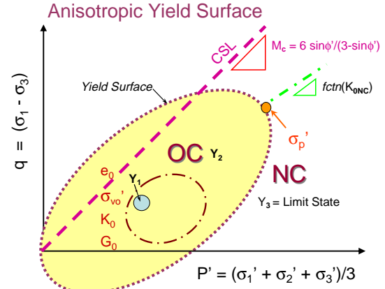
Figure 1.38. Anisotropic yield surface with zone Y1 for small-strain stiffness (after Jardine et al. 2005).
