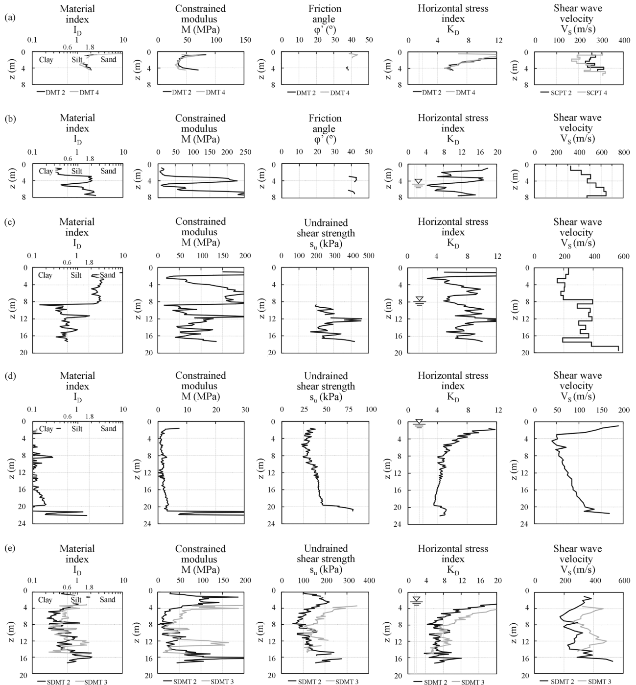
Figure 14 - DMT profiles and V_s profiles at different sites in Western Australia: (a) Shenton Park, (b) Ledge Point, (c) Perth CBD, (d) East Perth, (e) Margaret River (Amoroso, 2011).
