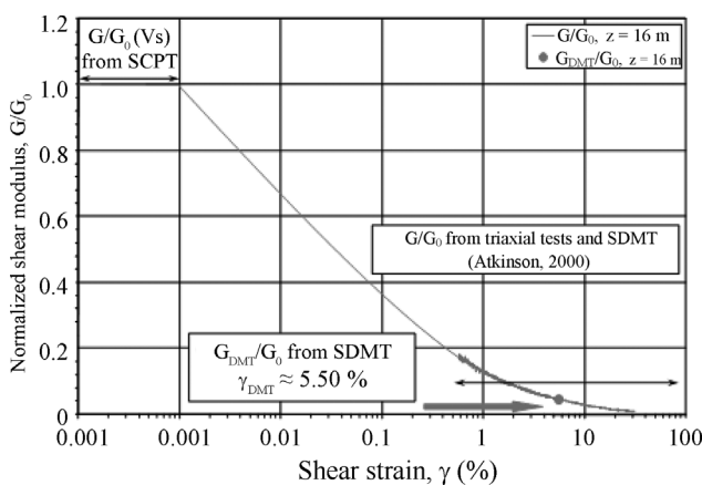
Figure 18 - In situ G/G_0 - \gamma decay curves and superimposed G_{DMT}/G_0 data points at East Perth (soft clay), Western Australia (Amoroso et al. , 2012).
