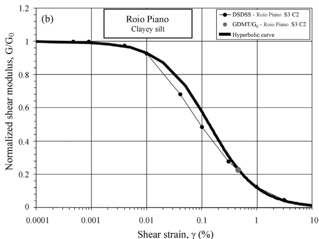
Figure 23 - Comparison between hyperbolic and “measured” stiffness decay curves at Shenton Park (a) and Roio Piano (b).
