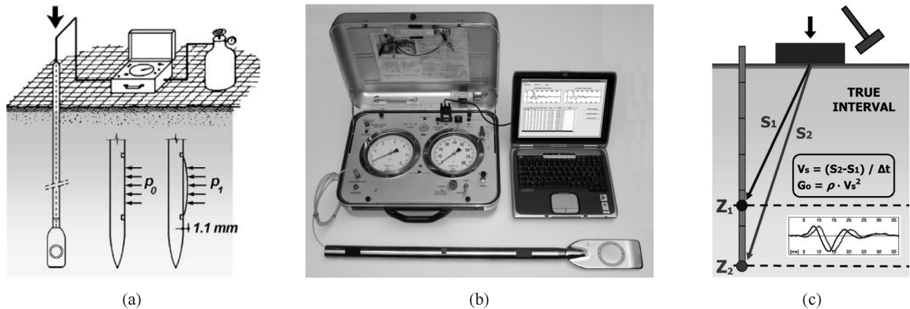
Figure 1 - (a) Schematic layout of the flat dilatometer test. (b) Seismic dilatometer equipment. (c) Schematic layout of the seismic dilatometer test (Marchetti et al. , 2001; Marchetti et al. , 2008).
