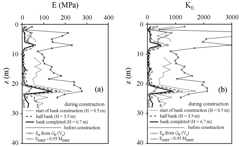
Figure 4 - Variation of (a) secant Young's modulus E , and (b) corresponding modulus number K_E (Eq. 2), back-calculated from local \varepsilon_v measured at the center under various embankment loads throughout construction (Monaco et al. , 2014, with permission from ASCE).
