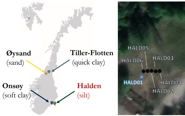
Figure 2. Location of Medusa (S)DMT (HALD02–HALD06) and traditional SDMT (HALD01) at Halden.
