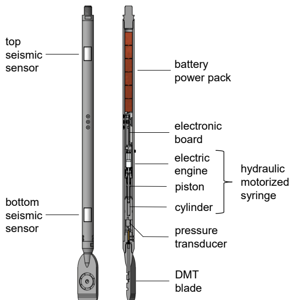
Figure 1. Medusa SDMT equipment.
