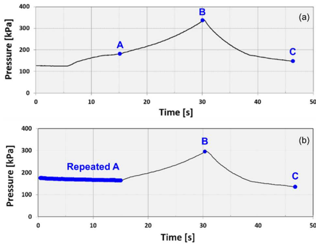
Figure 3. Medusa DMT test cycles (pressure vs. time and A, B, C readings) obtained at Fucino-Telespazio by: (a) Standard DMT procedure (STD), sounding Medusa 1, depth 8 m, (b) DMT Repeated A-readings procedure (DMT-RA), sounding Medusa 2, depth 8 m.
