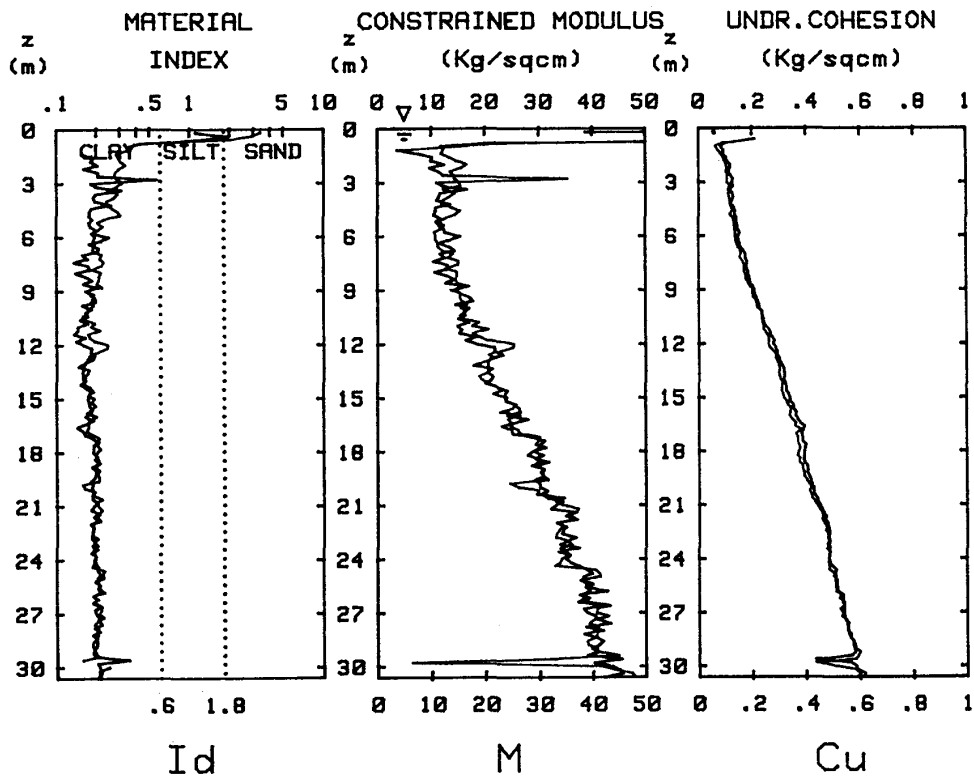
Example of repeatability of DMT results Operators : Cestari (SGI), Lacasse (NGI), Lunne (NGI), Marchetti (Aq) Marine NC sensitive clay (Onsoy, Norway)
