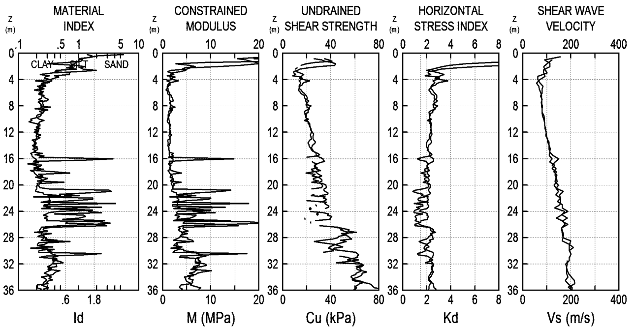
Example of repeatability of SDMT results
