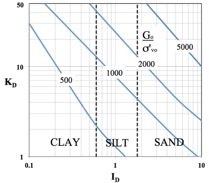
Fig. 7. Contours of G_o/\sigma'_{vo} plotted on modified DMT-based chart for soil type based on I_D and K_D (based on Marchetti, 2014)
