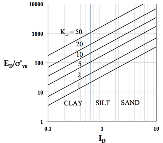
Fig. 4. Modified DMT-based chart for soil type based on dimensionless I_D and E_D/\sigma'_{vo}
