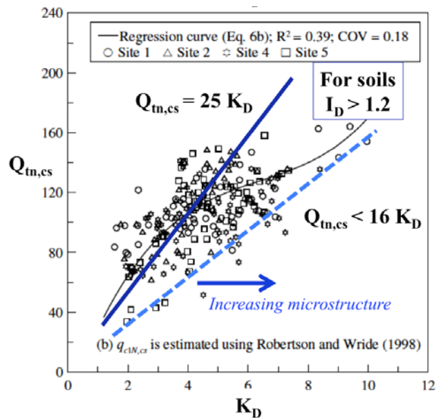
Fig. 9. Relationship between CPT Q_{m,cs} and K_D for young, uncemented sandy soils ( I_D > 1.2 ) (data from Tsai et al, 2009)
