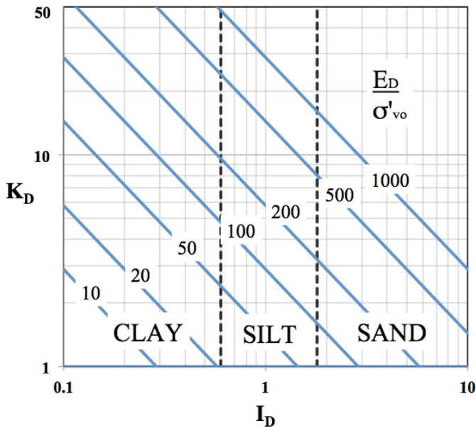
Fig. 5. Proposed modified DMT-based chart for soil type based on I_D and K_D
