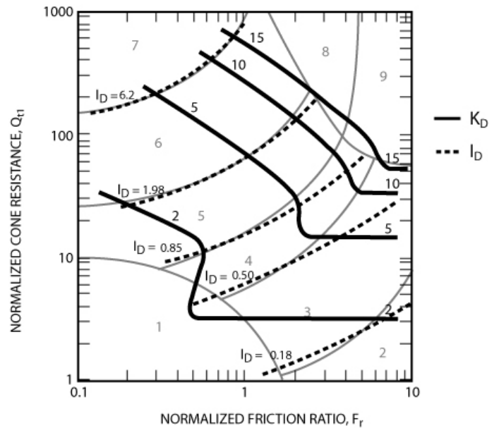
Fig. 2. Approximate correlation between DMT K_D and I_D and CPT normalized parameters for soils with little or no microstructure (After Robertson, 2010)
