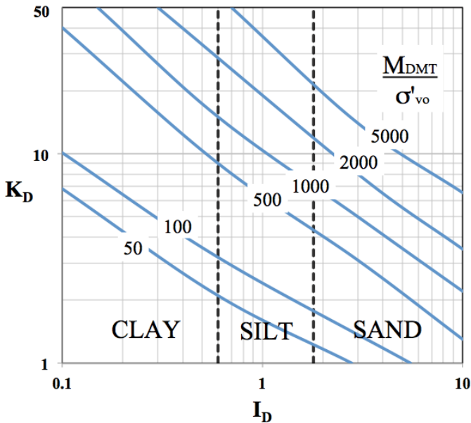
Fig. 6. Contours of M_{DMT}/\sigma'_{vo} plotted on modified DMT-based chart for soil type based on I_D and K_D (based on Marchetti, 1980)
