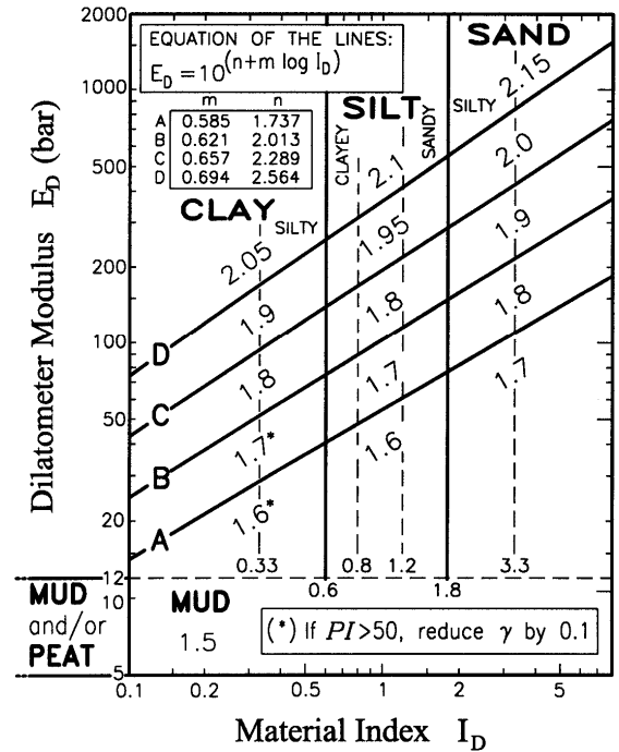
Fig. 3. DMT-based chart for soil type and unit weight based on I_D and E_D (After Marchetti and Crapps, 1981)
