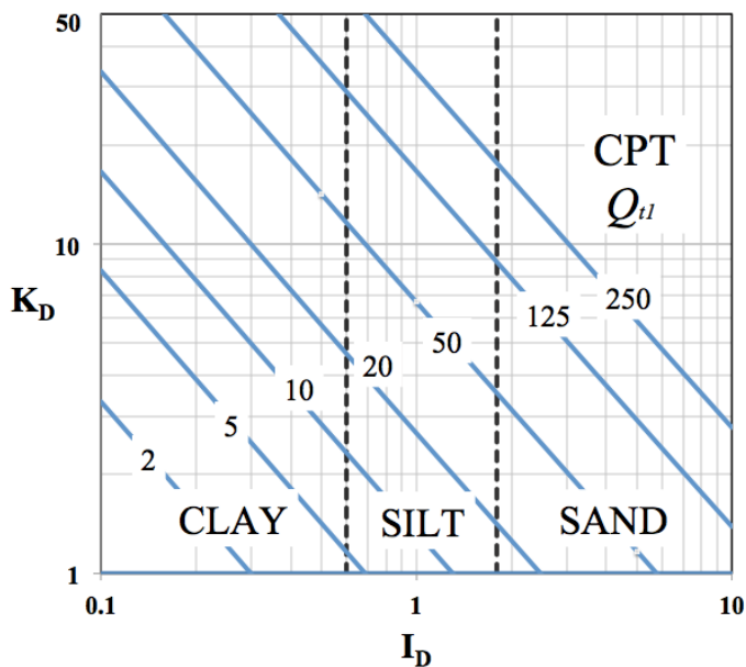
Fig. 10. Simplified link between CPT Q_{t1} and DMT K_D - I_D for young, uncemented soils Q_{t1} = (1.5 \log I_D + 7.5) I_D K_D
