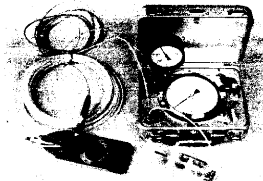
Figure 3. Calibration equipment for dilatometer membranes.
