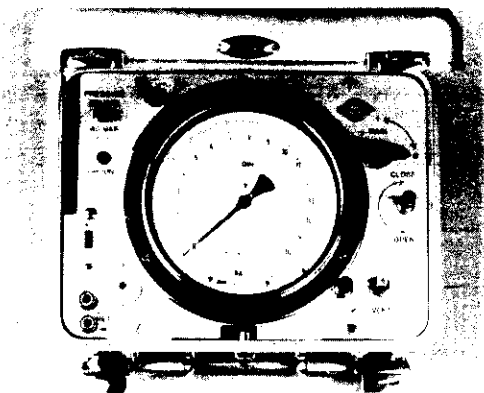
Figure 2. Regulation unit for dilatometer.
