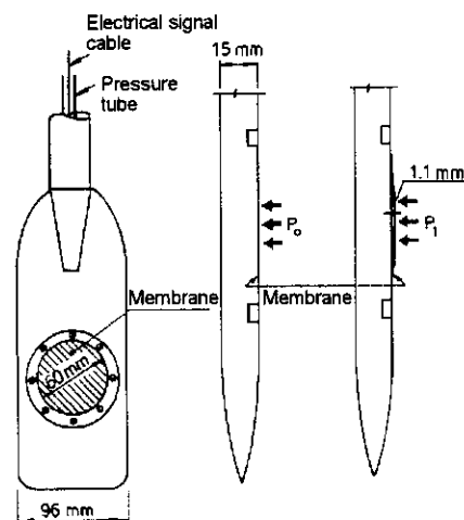
Figure 1. The dilatometer.
