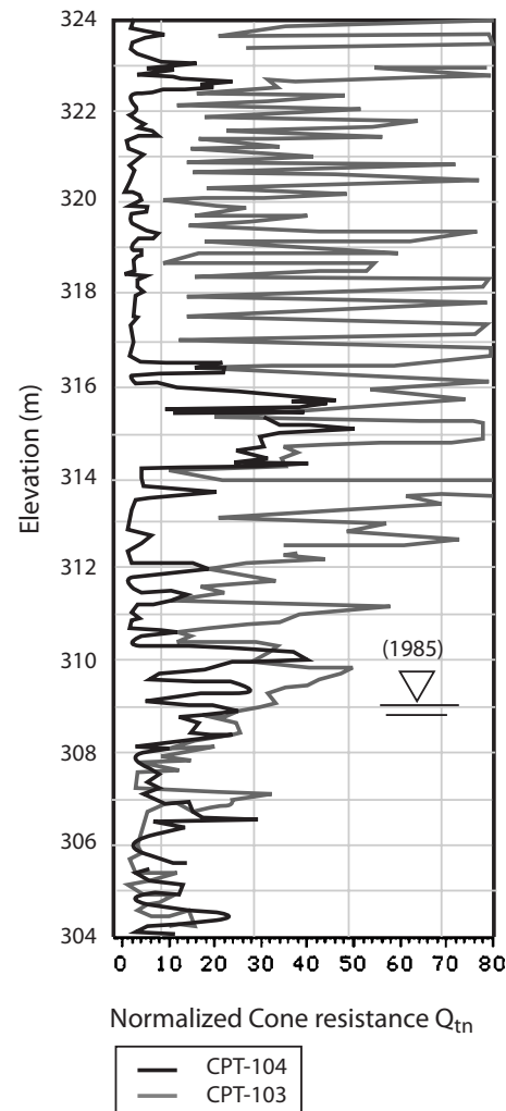
Fig. 2. LSFDF CPT profiles (C103 and C104)
