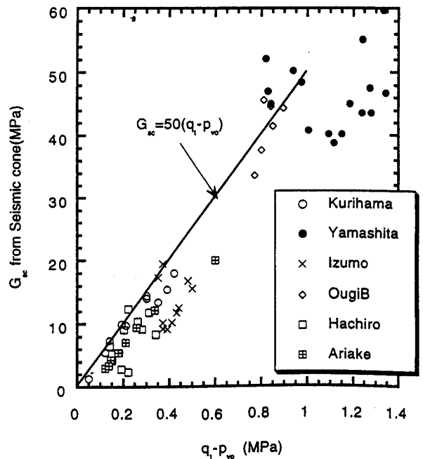
Fig. 17. Correlation of G_{sc} from seismic cone and (q_t - p_{v0}) from CPT for clays after Tanaka et al. (1994) (some data are added to the original diagram)
