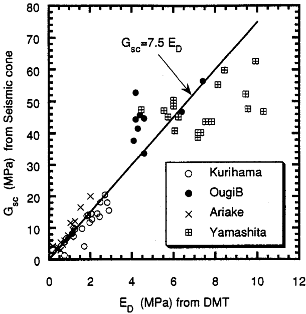
Fig. 18. Correlation of G_{sc} from seismic cone and E_D from DMT for clays after Tanaka et al. (1994) (some data are added to the original diagram)
