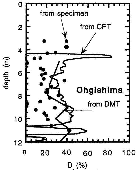
Fig. 14. Relative density against depth at Ohgishima
