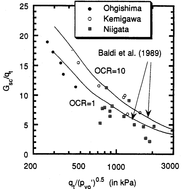
Fig. 20. Correlation of G_{sc}/q_t and q_t/(p'_{v0})^{0.5}
