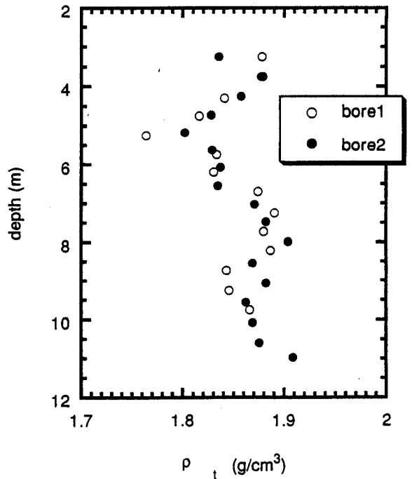
Fig. 5. Average of unit soil mass for 0.5 m depth (Ohgishima)
