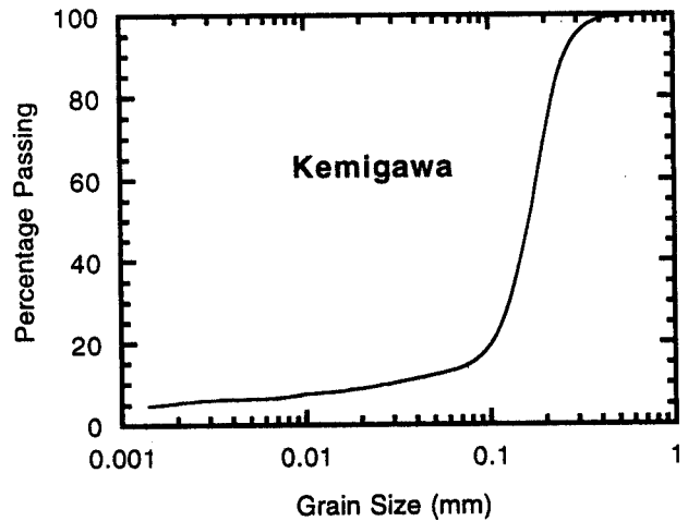
Fig. 9. Gradation curve of the objective layer at Kemigawa
