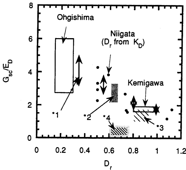
Fig. 21. Correlation with G_{sc}/E_D and D_r .
