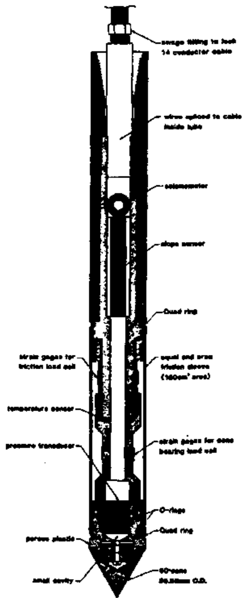
Fig. 1. Seismic Cone Penetrometer.
