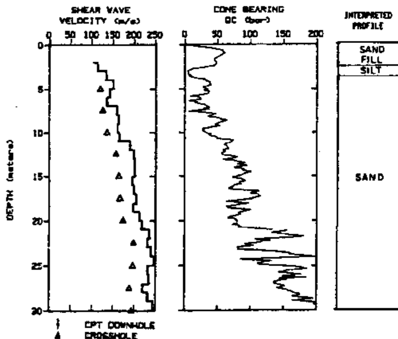
Fig. 7. Comparison of Seismic CPT Downhole and Crosshole Data at Anacis Site, Vancouver.
